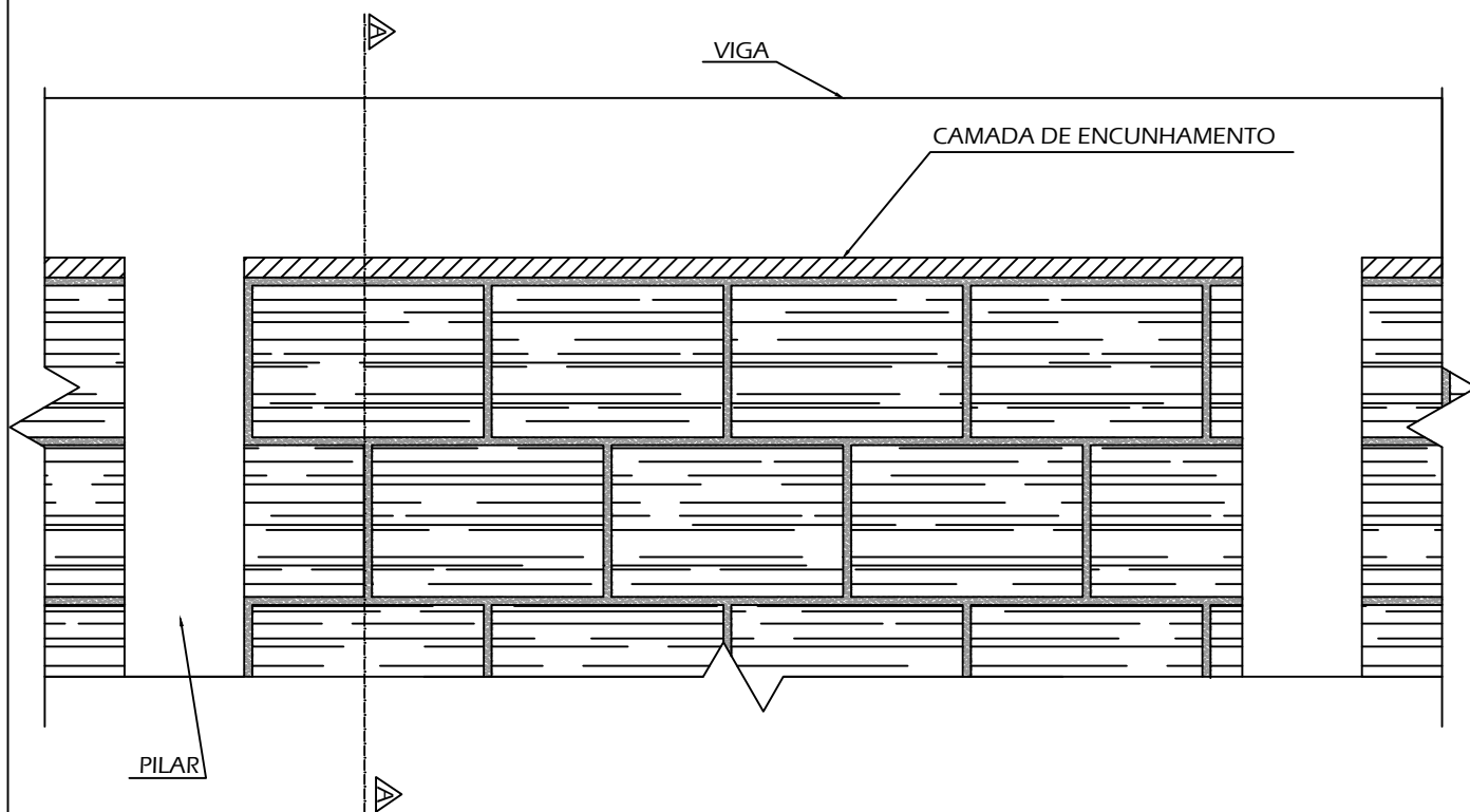
VISTA FRONTAL
