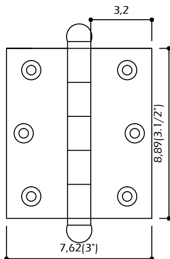
DOBRADIÇA 3.1/2"x 3"
